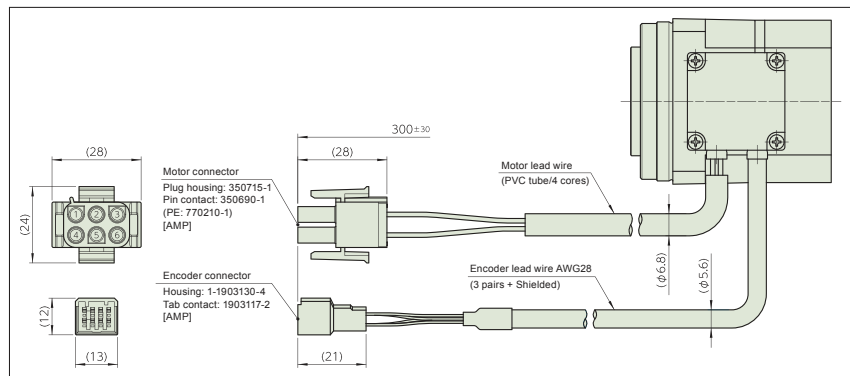
Lead wire of the motor and encoder (common to all models)
